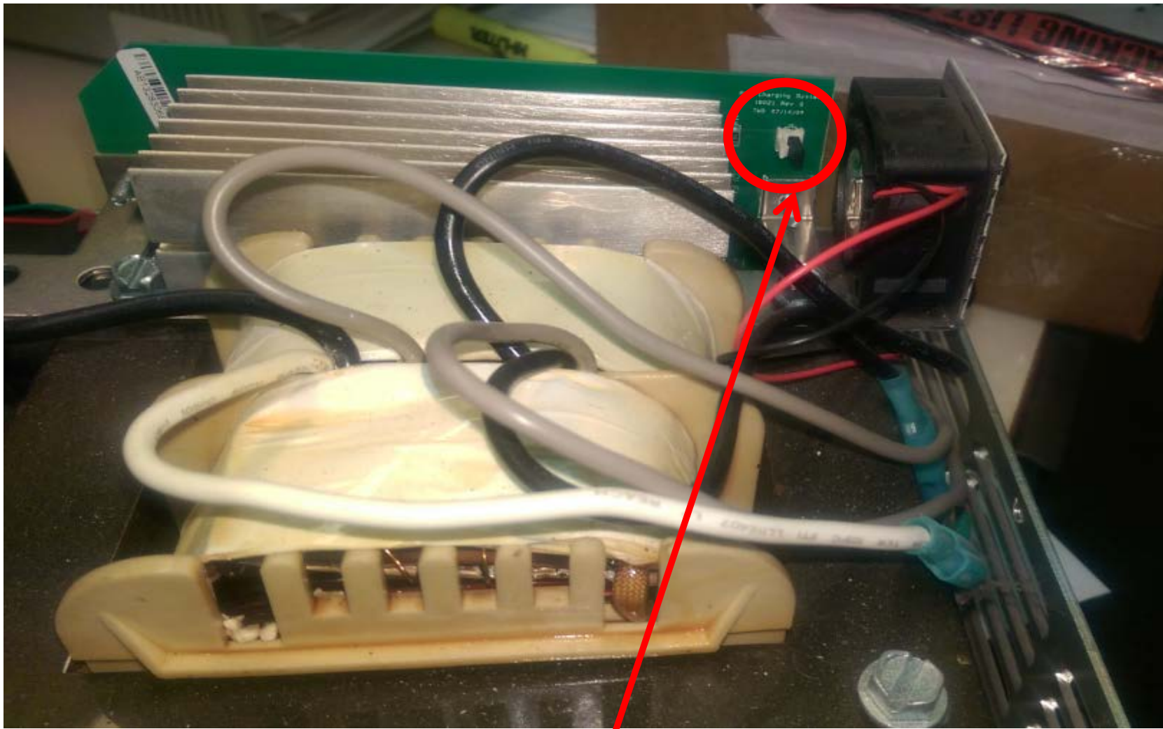
Charger is set for GEL/AGM Jumper is set on pins
